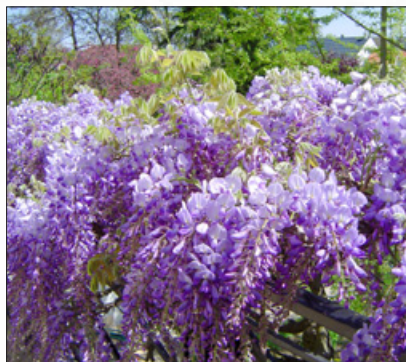
Glycine |
